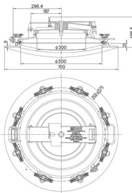
Fitting Details
