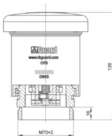
Fitting Details
